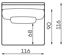
1,5-SEATER
